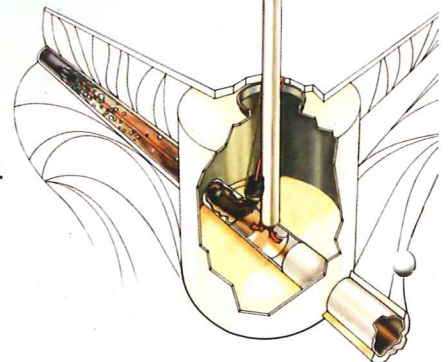
Vacuum power with precise jet-rodding action to remove solid and liquid debris from your entire waste water collection system or treatment facility.
